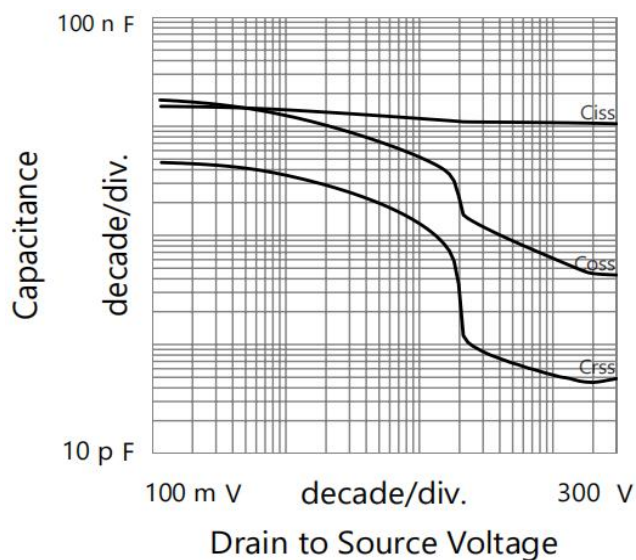
Fig 4. Capacitance Characteristics
