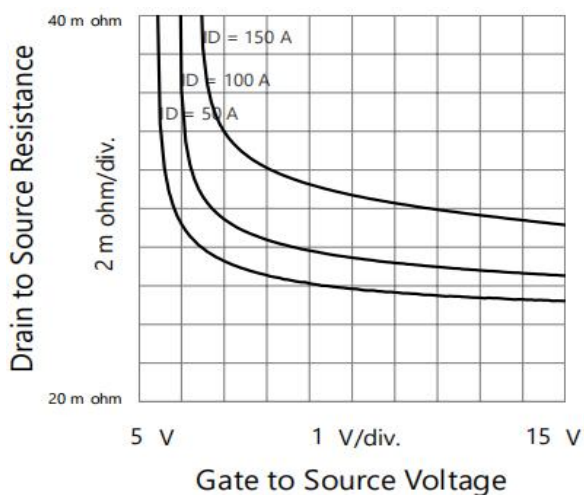
Fig 9 .Drain to Source Resistance vs. Gate to Source Voltage
