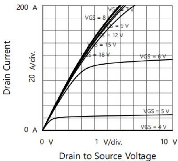
Fig1. Output characteristics TJ= 25°C
