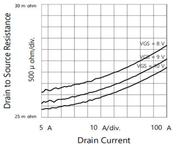
Fig 6. ID VS RDson
