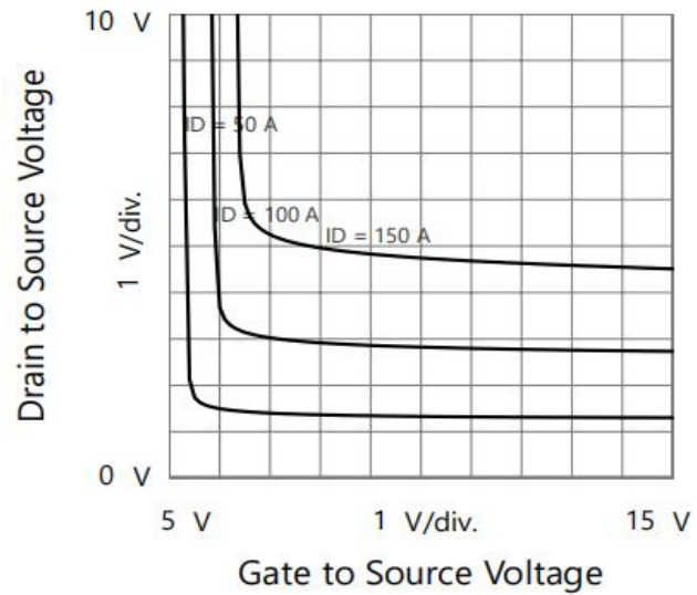
Fig 8 .Drain to Source Voltage vs. Gate to Source Voltage
