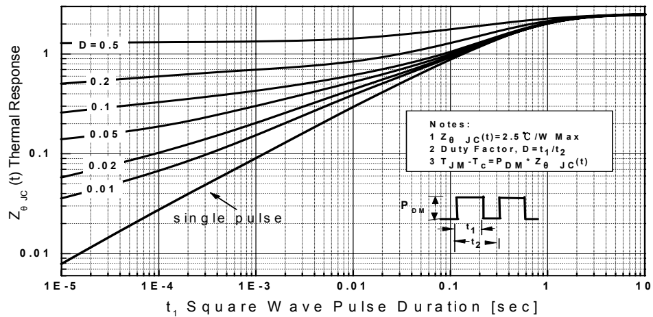
Transient Thermal Response Curve For 10N65F
