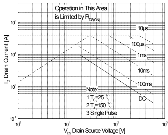
Maximum Safe Operating Area For 10N65C
