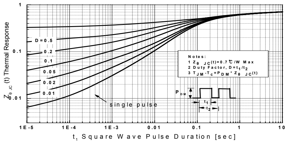
Transient Thermal Response Curve For 10N65C
