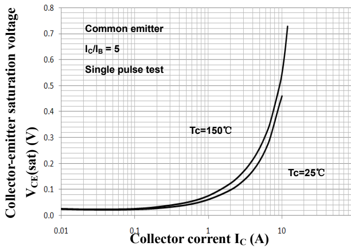
Saturation Voltage
