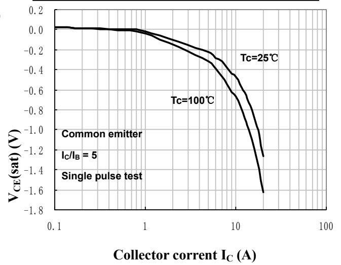
Saturation Voltage
