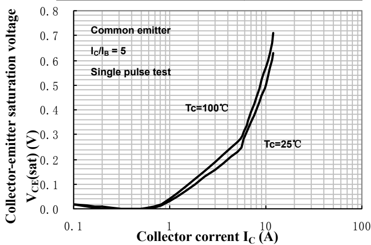
Saturation Voltage
