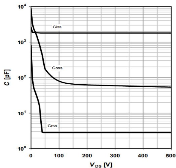
Fig 4. Capacitance Characteristics
