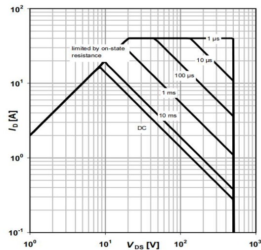
Fig 8 .Safe operating area
