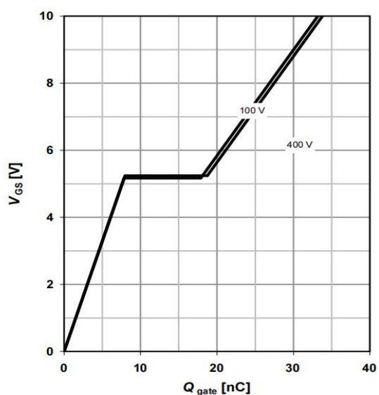
Fig3. Gate charge characteristics
