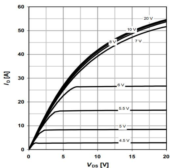
Fig1. Output characteristics T_J = 25^\circ\text{C}
