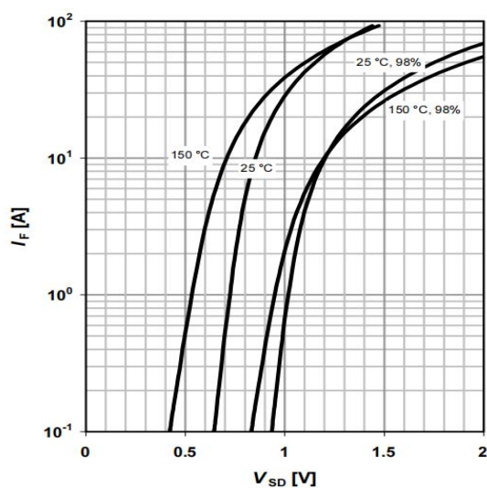
Fig 7 . Forward characteristics of reverse diode
