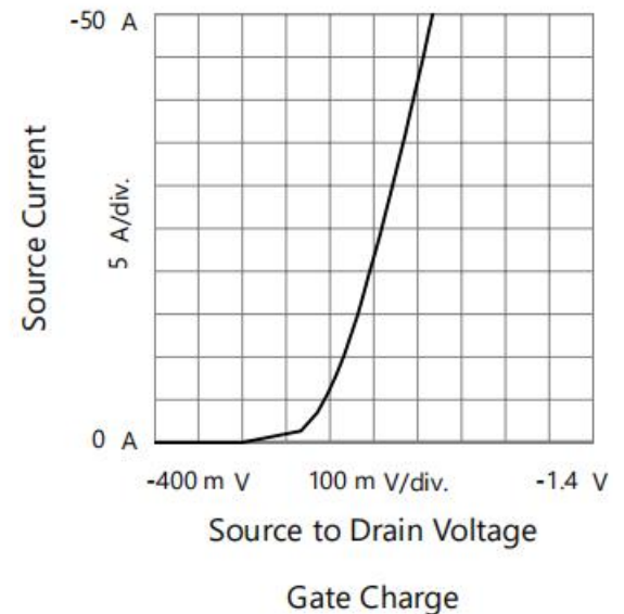
Body Diode Forward Characteristics
