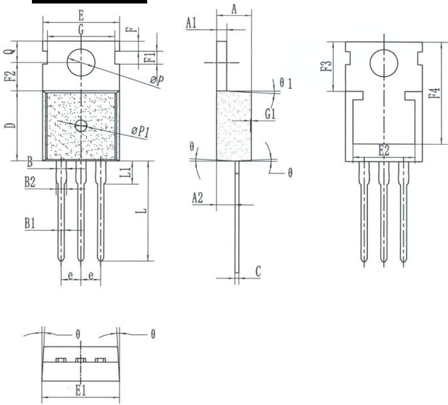
TO-220C
