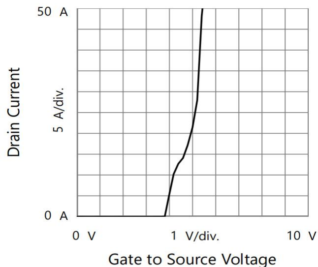
Fig2. Transfer characteristics
