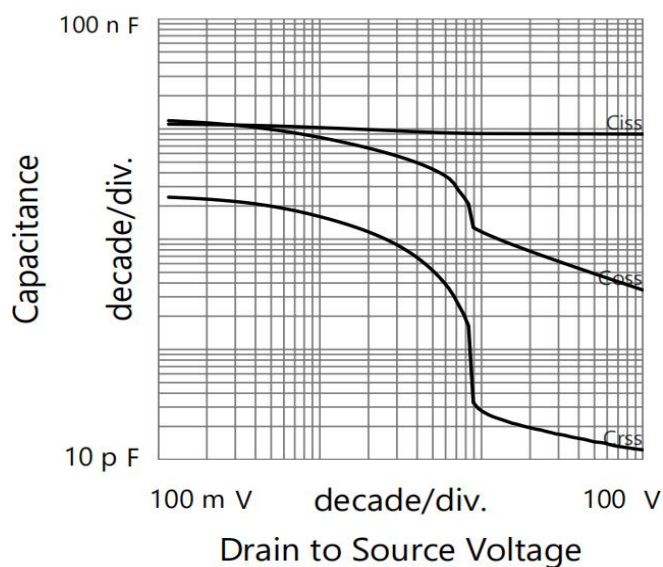
Fig 4. Capacitance Characteristics
