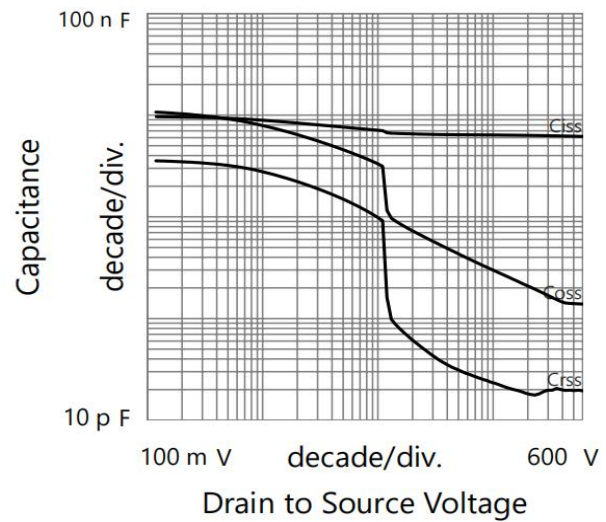
Fig 4. Capacitance Characteristics
