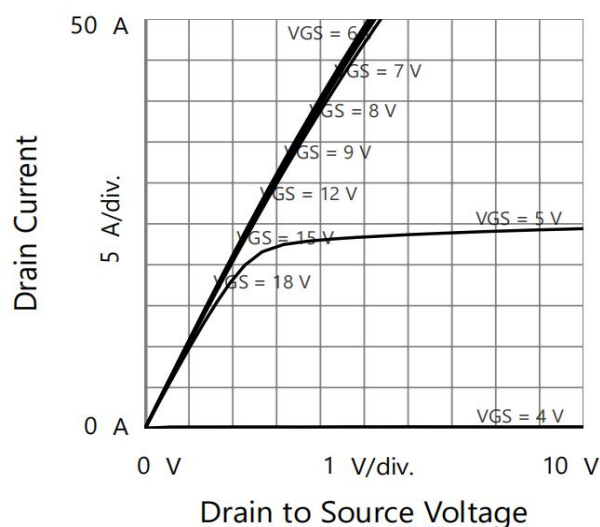
Fig1. Output characteristics TJ= 25°C
