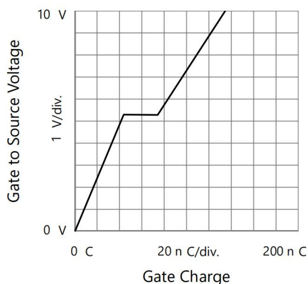
Fig3. Gate charge characteristics
