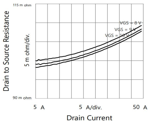
Fig 6. ID VS RDson
