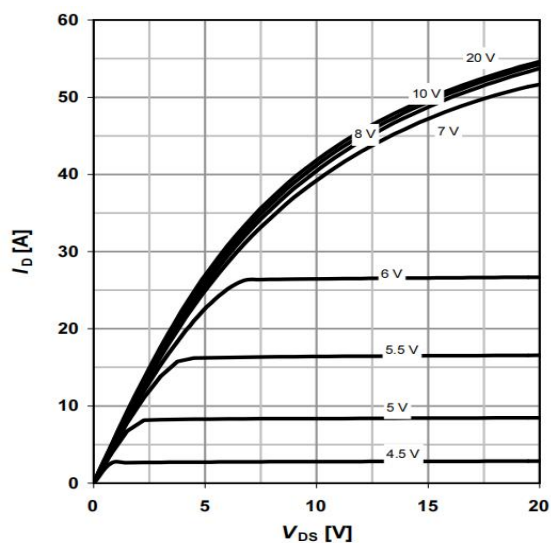
Fig1. Output characteristics TJ= 25°C
