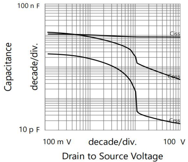
Fig 4. Capacitance Characteristics
