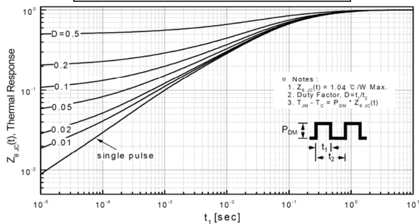
Transient Thermal Response Curve For 7N65F
