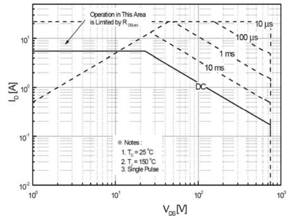
Maximum Safe Operating Area For 7N65F
