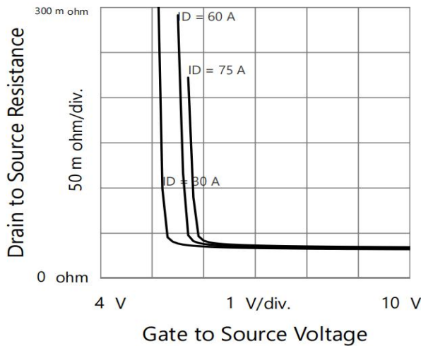
Gate to Source Voltage Fig 9 .Drain to Source Resistance vs. Gate to Source Voltage
