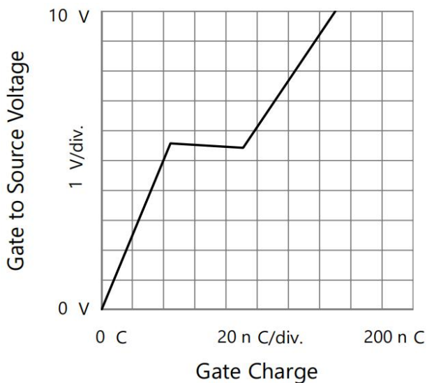
Fig3. Gate charge characteristics
