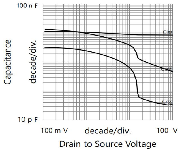
Fig 4. Capacitance Characteristics
