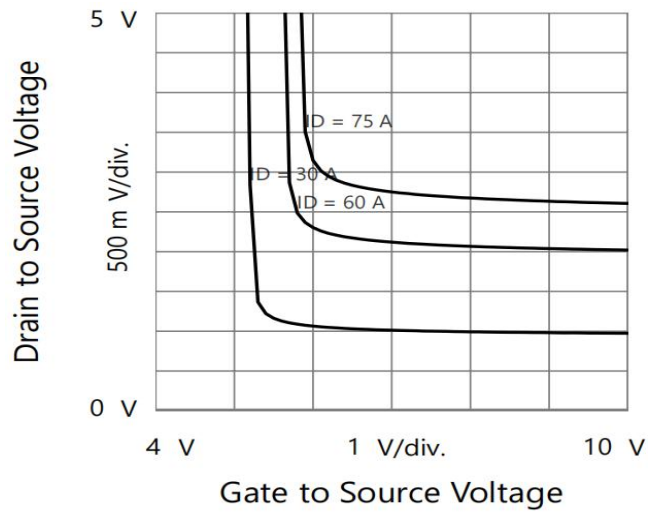
Gate to Source Voltage Fig 8 .Drain to Source Voltage vs. Gate to Source Voltage
