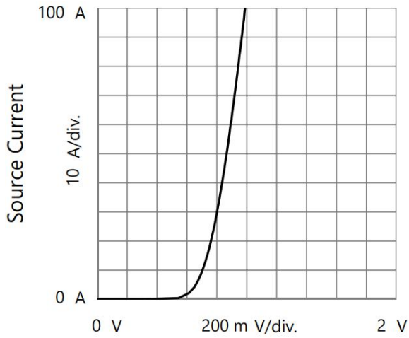
Source to Drain Voltage Fig 7 . Forward characteristics of reverse diode
