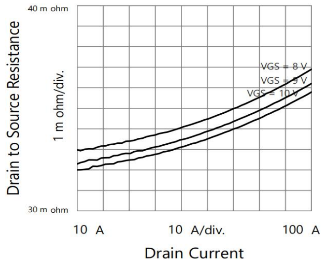
Fig 6. I_D VS R_{Dson}
