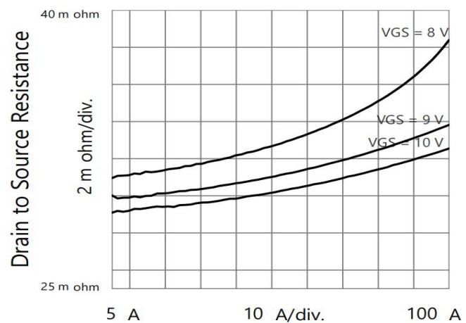
Drain Current
