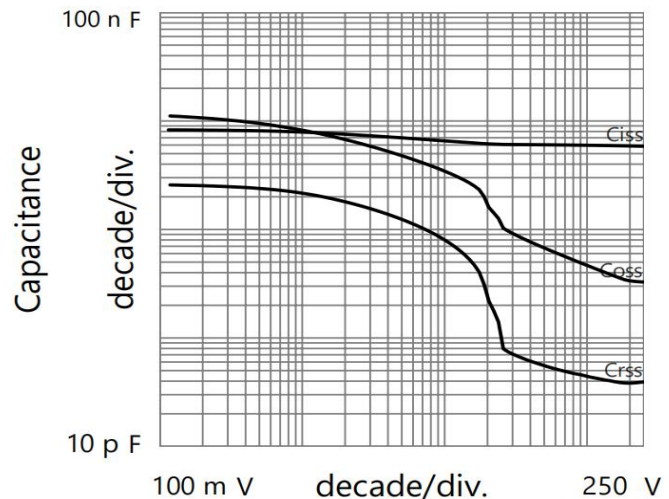
Drain to Source Voltage
