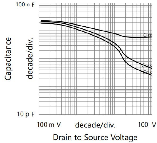
Fig 8 .Capacitances
