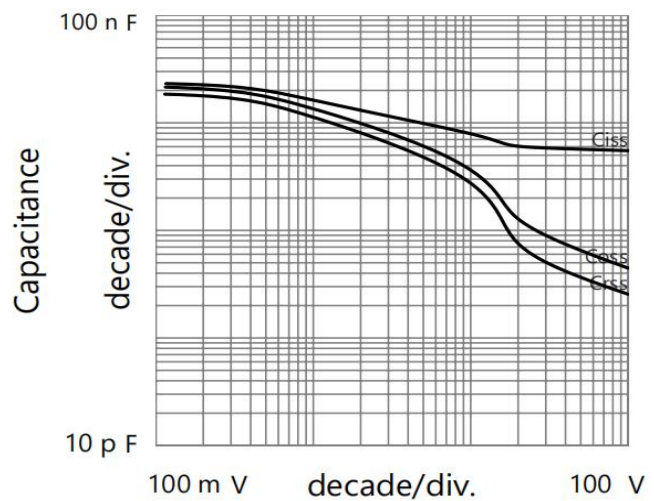
Drain to Source Voltage Fig 4. Capacitance Characteristics
