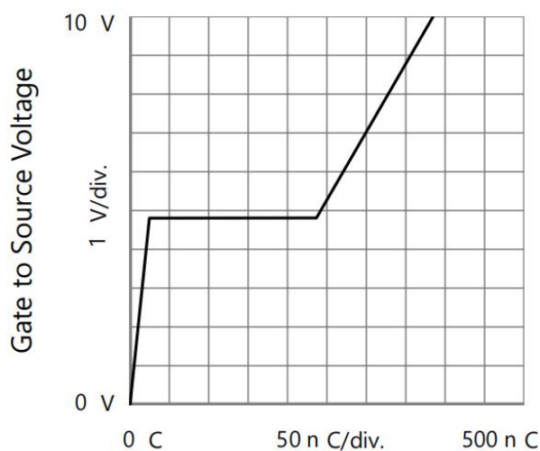
Gate Charge Fig3. Gate charge characteristics
