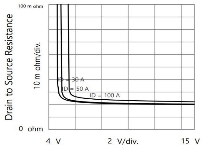
Gate to Source Voltage Fig 6. Drain to Source Resistance vs. Gate to Source Voltage
