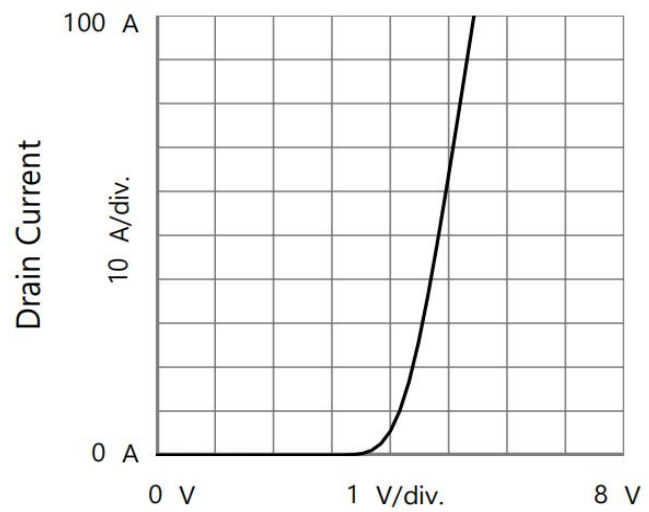
Gate to Source Voltage Fig2. Transfer characteristics
