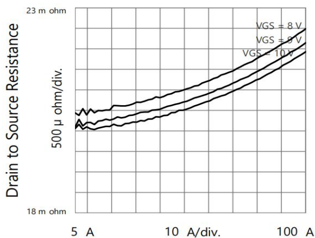
Drain Current Fig 5. Drain to Source Resistance vs. Drain Current
