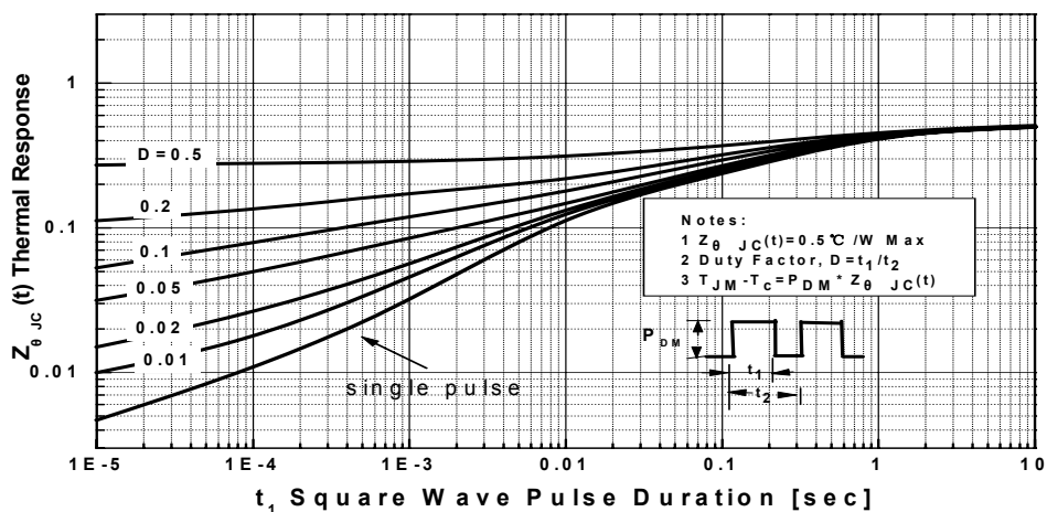
Transient Thermal Response Curve For 13N65C
