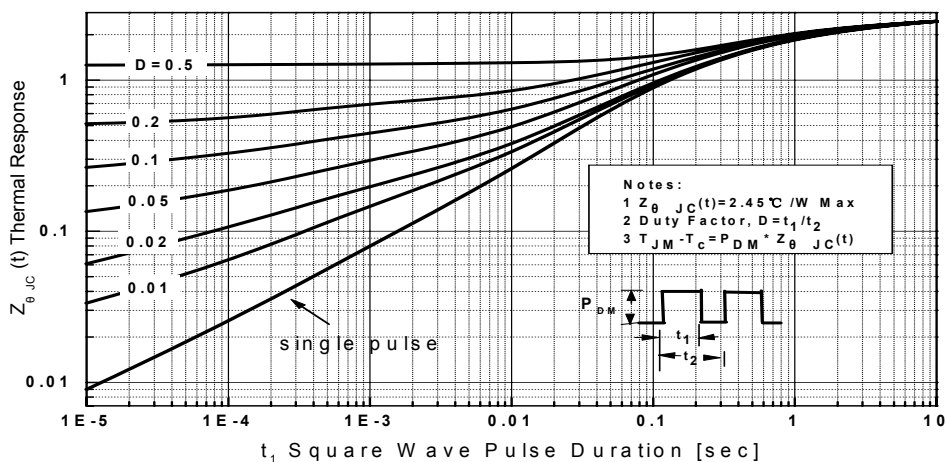
Transient Thermal Response Curve For 13N65F
