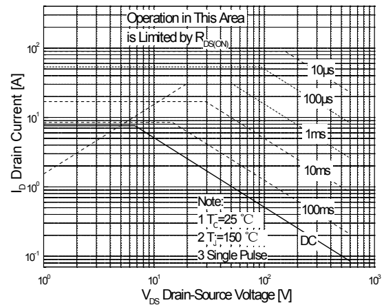
Maximum Safe Operating Area For 12N65F
