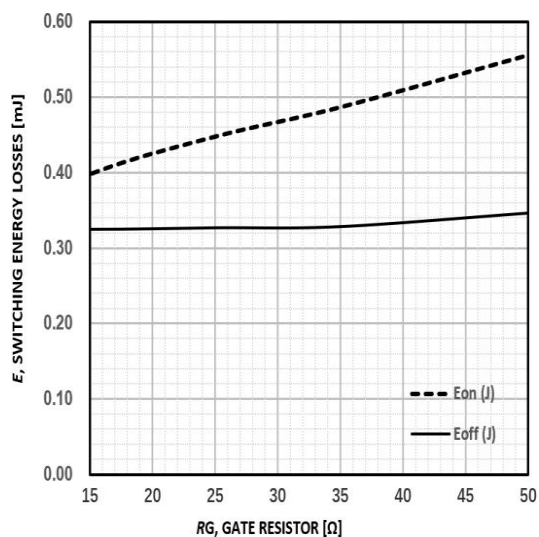
Figure 9. Typical energy loss VS. R_g , T_C=25^\circ\text{C} , V_{CE}=400\text{V} , V_{GE}=15\text{V} , I_C=15\text{A}
