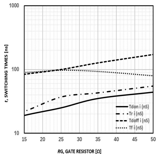
Figure 10. Typical switching time VS. R_g , T_C=25^\circ\text{C} , V_{CE}=400\text{V} , V_{GE}=15\text{V} , I_C=15\text{A}
