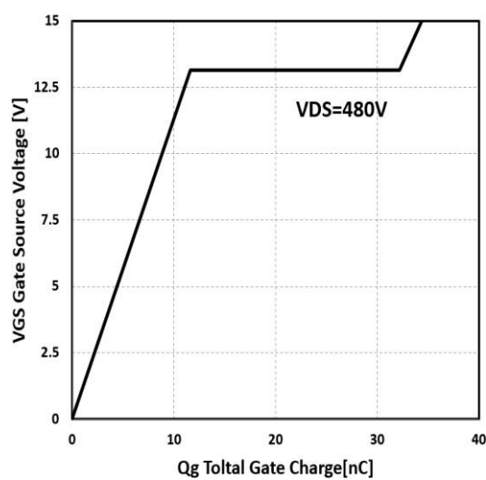
Figure 4. Typical gate charge VS. V_{GE} , I_C=15\text{A}
