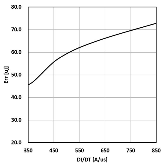
Figure 16. Typical diode Err vs di/dt Tc=25°C VCE=400V VGE=15V IF=15A
