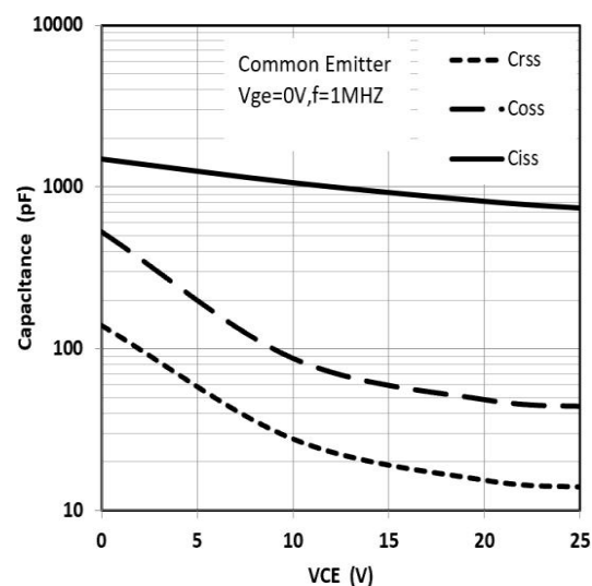
Figure 6. Typical capacitance VS. VCE, V_{GE}=0V, f=1MHz
