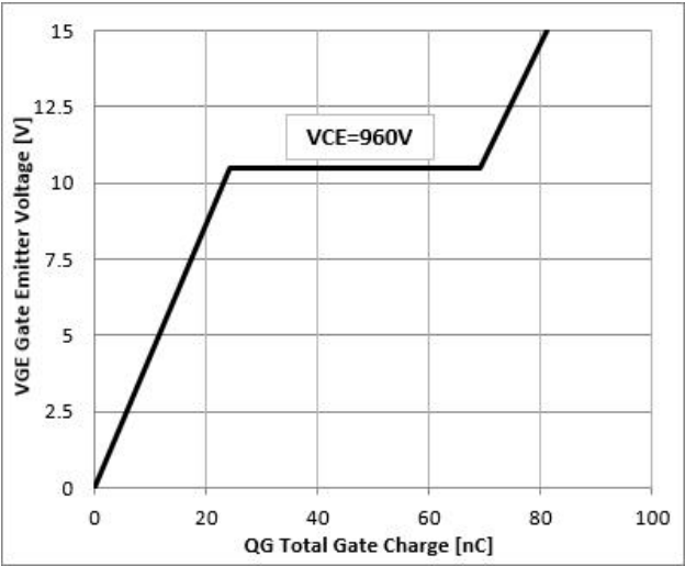
Figure 4: Typical Gate charge VS. VGE,IC=15A
