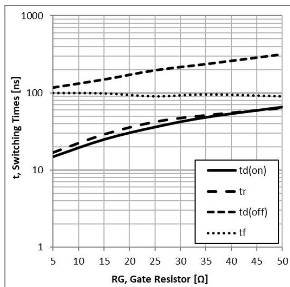
Figure 10: Typical Switching Time VS. RG, TC=25°C, L=200uH, VCE=600V, VGE=15V, IC=15A
