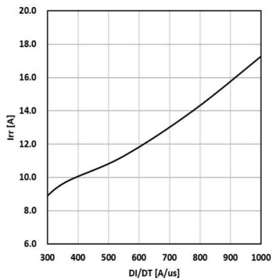
Figure 14. Typical diode Irr vs di/dt Tc=25°C VCE=600V VGE=15V IF=15A
