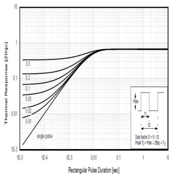
Figure18. normalized transient thermal impedance, junction-to-case
