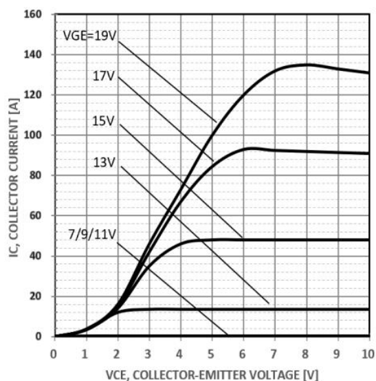
Figure 5. Typical output characteristics t_p=300\mu s T_c=25^\circ C
