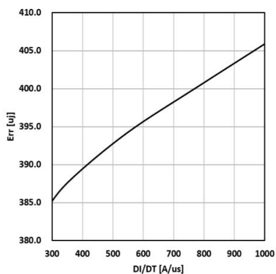
Figure 16. Typical diode Err vs di/dt Tc=25°C VCC=600V VGE=15V IF=15A
