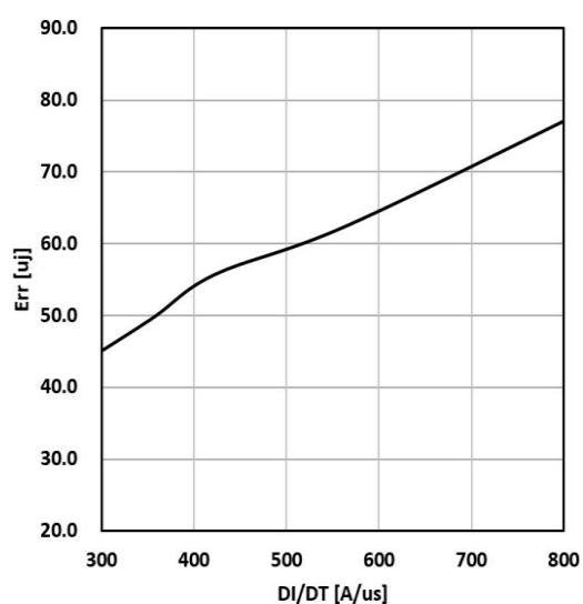
Figure 16. Typical diode Err vs di/dt Tc=25°C VCE=400V VGE=15V IF=20A
