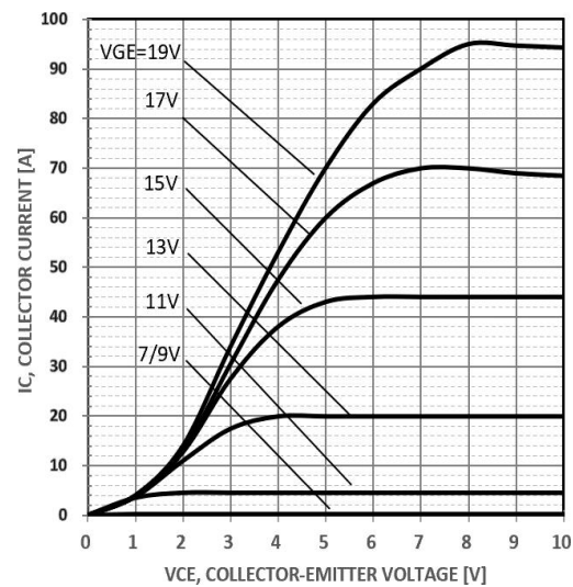
Figure 6. Typical output characteristics t_p=300\mu s T_c=150^\circ C
