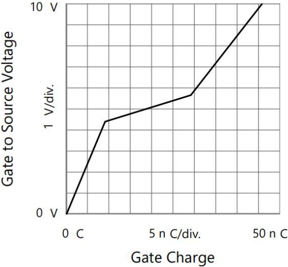
Figure 8. Gate Charge
