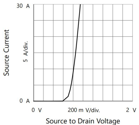
Figure 6. Body Diode Forward Characteristics
