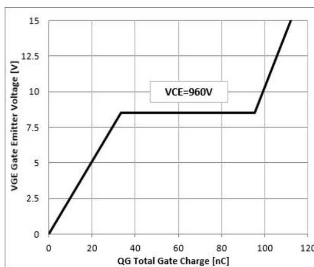
Figure 4: Typical Gate charge VS. V_{GE} , I_C=25\text{A}
