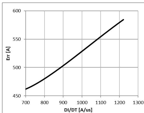
Figure 16: Typical Diode Err VS. DI/DT, TC=25°C VCC=600V, VGE=15V, IF=25A
