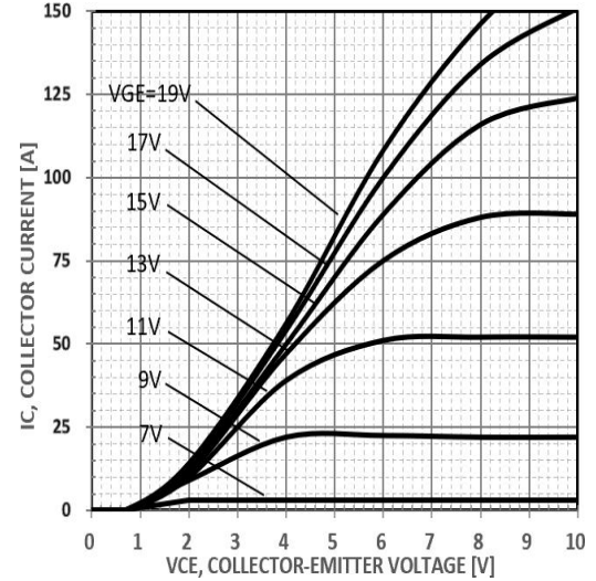
Figure 6. typical IGBT output characteristics, T_J=150^{\circ}\text{C} ; t_p=300\mu\text{s}
