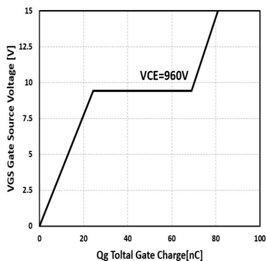
Figure 4. Typical gate charge VS. V_{GE} , I_C=25\text{A}
