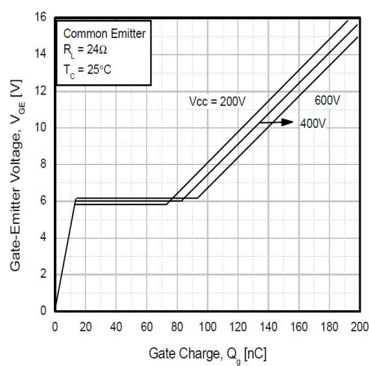
Figure4: Typical gate charge VS. V_{GE} , I_C=25\text{A}
