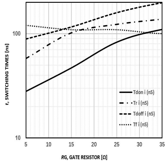
Figure10: Typical switching time VS. R_g , T_C=25^\circ\text{C} , V_{CE}=600\text{V} , V_{GE}=15\text{V} , I_C=25\text{A}
