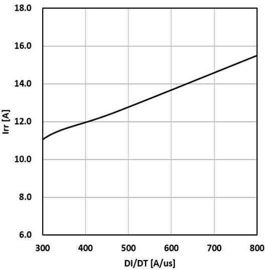
Figure 14. Typical diode irr vs di/dt Tc=25℃ VCE=600V VGE=15V IF=25A
