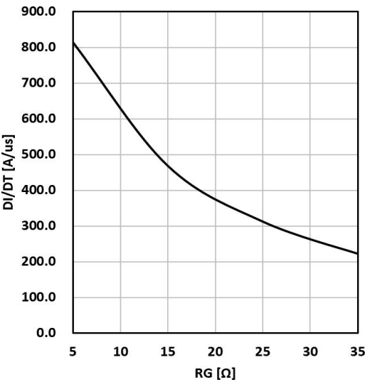
Figure 13. Typical diode di/dt vs rg Tc=25℃ VCE=600V VGE=15V IF=25A
