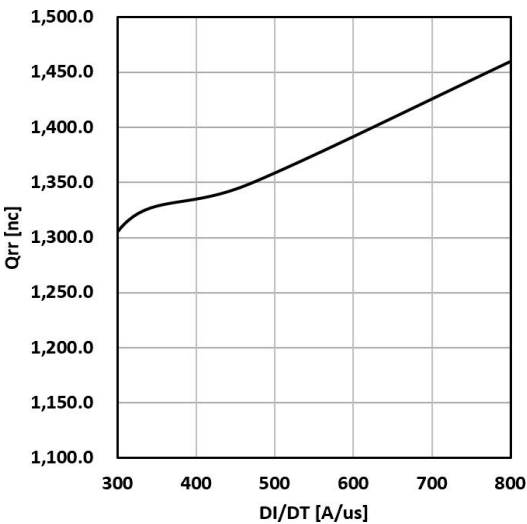
Figure 15. Typical diode Qrr vs di/dt Tc=25℃ VCE=600V VGE=15V IF=25A
