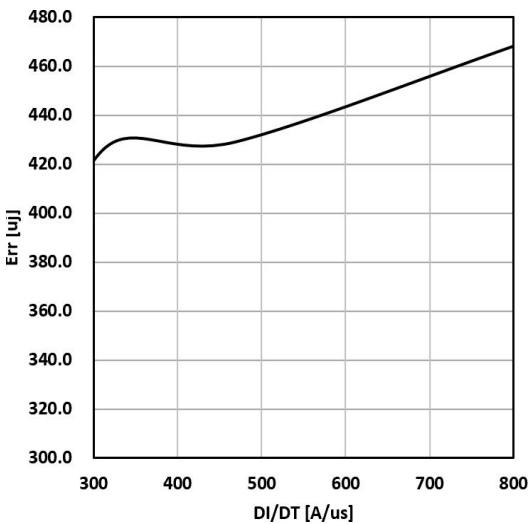
Figure 16. Typical diode Err vs di/dt Tc=25℃ VCC=600V VGE=15V IF=25A
