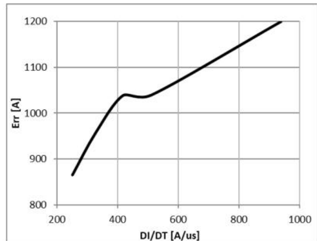
Figure 16: Typical Diode Err VS. DI/DT, TC=25°C VCC=600V, VGE=15V, IF=40A
