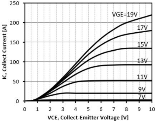
Figure 6: Typical IGBT Output characteristics, C=150°C; tp=300us
