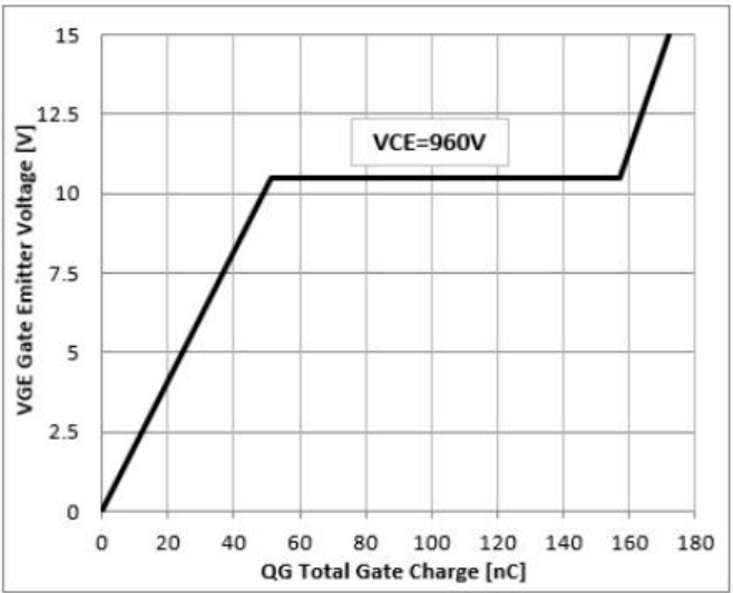
Figure 4: Typical Gate charge VS. VGE, IC=40A
