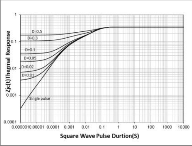
Figure 18: Normalized transient thermal impedance junction-to-case
