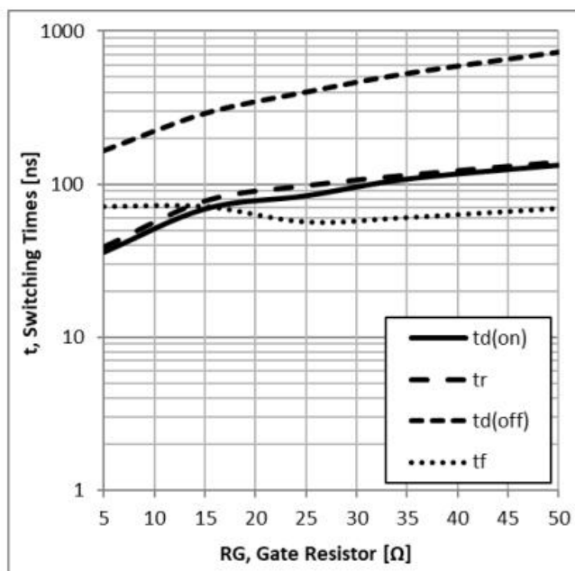
Figure 10: Typical Switching Time VS. RG, TC=25°C, L=200uH, VCE=600V, VGE=15V, IC=40A
