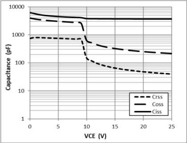
Figure 17: Typical Capacitance VS. VCE, VGE=0V,f=1MHz
