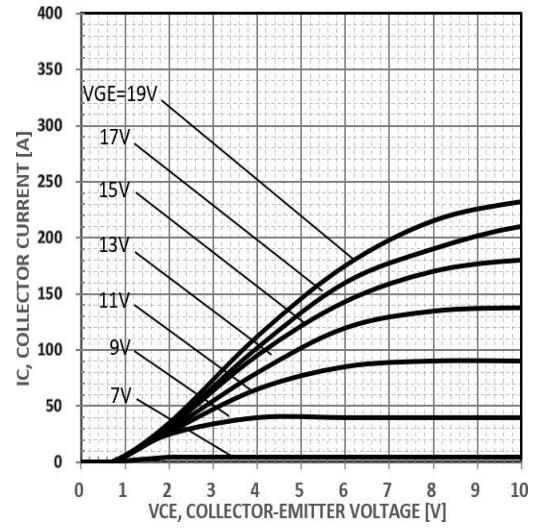
Figure 6. Typical output characteristics tp=300us Tc=150°C
