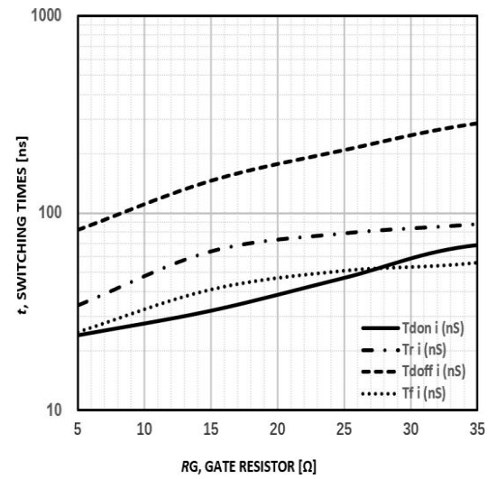
Figure10: Typical switching time VS. Rg, TC=25°C, VCE=400V, VGE=15V, IC=40A
