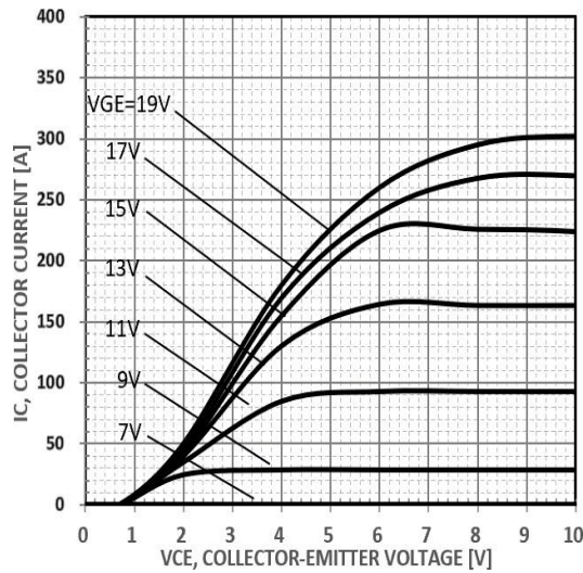
Figure 5. Typical output characteristics tp=300us Tc=25°C
