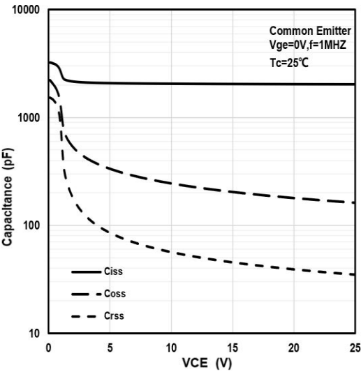
Figure17:Typical capacitance VS. VCE, VGE=0V,f=1MHz
