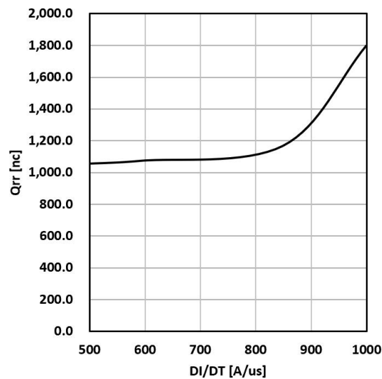
Figure 15. Typical diode Qrr vs di/dt Tc=25℃ VCE=400V VGE=15V IF=40A
