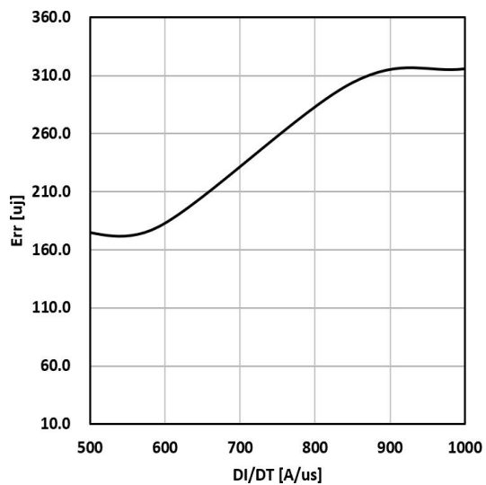
Figure 16. Typical diode Err vs di/dt Tc=25℃ VCC=400V VGE=15V IF=40A
