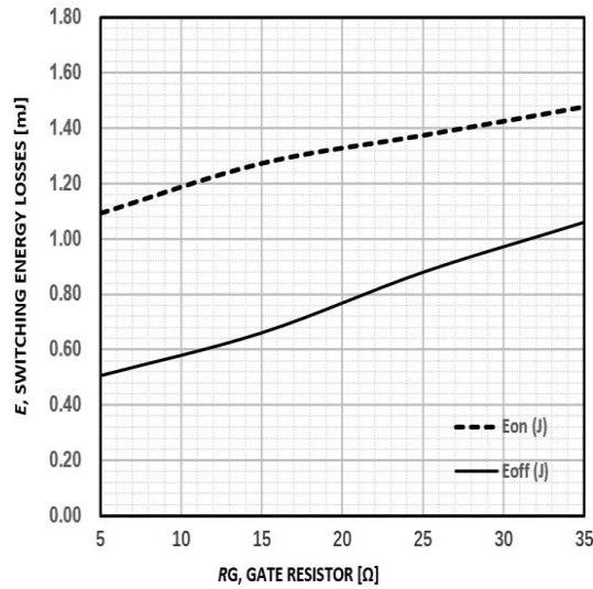
Figure9: Typical energy loss VS. Rg, TC=25°C, VCE=400V, VGE=15V, IC=40A
