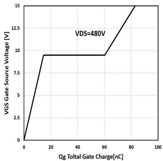
Figure 4: Typical gate charge VS. VGE, IC=40A
