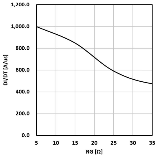
Figure 13. Typical diode di/dt vs rg Tc=25℃ VCE=400V VGE=15V IF=40A
