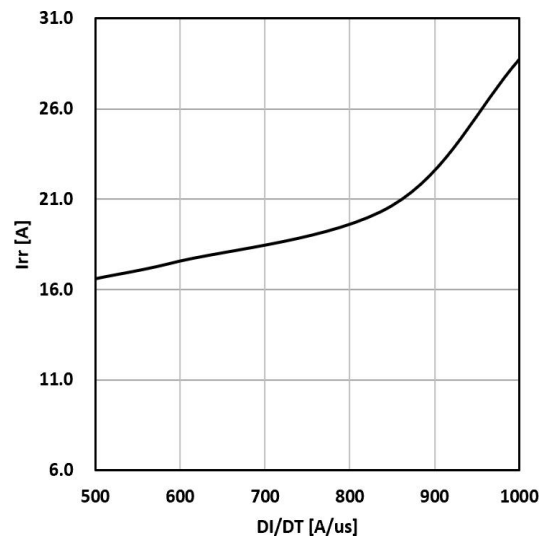
Figure 14. Typical diode irr vs di/dt Tc=25℃ VCE=400V VGE=15V IF=40A
