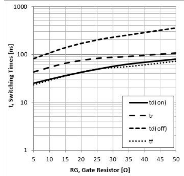
Figure 10: Typical Switching Time VS. RG, TC=25°C, L=100uH, VCE=400V, VGE=15V, IC=40A
