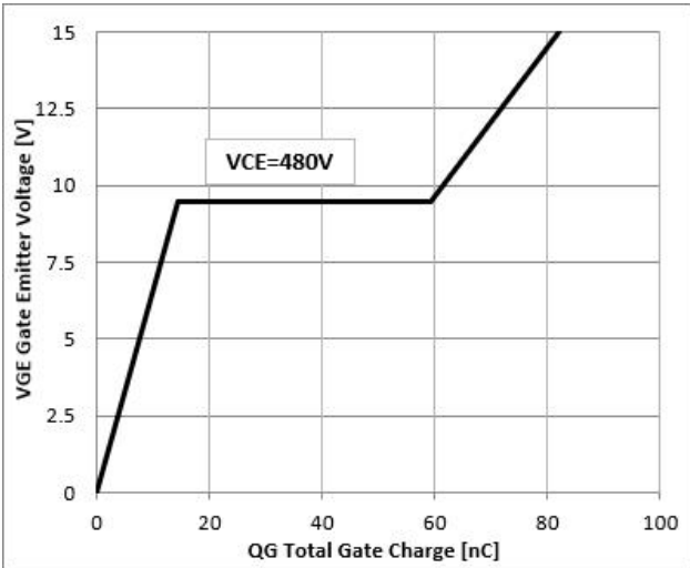
Figure 4: Typical Gate charge VS. VGE, IC=40A
