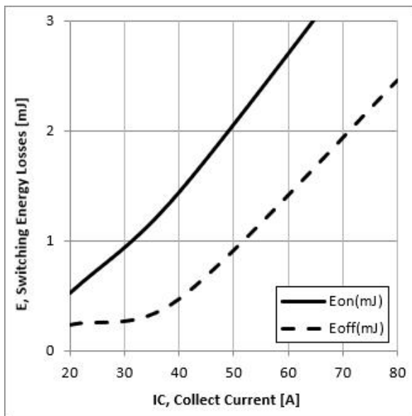
Figure 11: Typical Energy Loss VS. IC, TC=25°C, L=100uH, VCE=400V, VGE=15V, RG=15Ω
