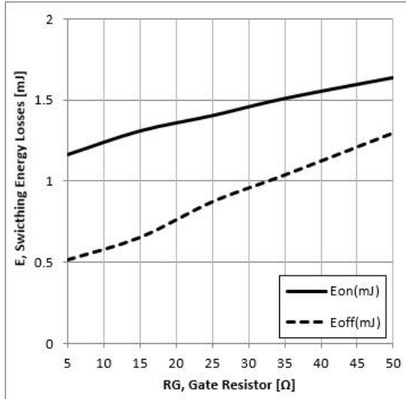
Figure 9: Typical Energy Loss VS. RG, TC=25°C, L=100uH, VCE=400V, VGE=15V, IC=40A
