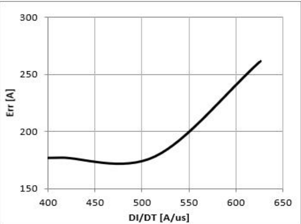
Figure 16: Typical Diode Err VS. DI/DT, TC=25°C VCC=400V, VGE=15V, IF=40A
