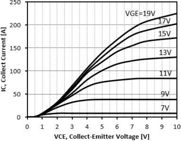
Figure 6: Typical IGBT Output characteristics, TC=150°C; tp=300us
