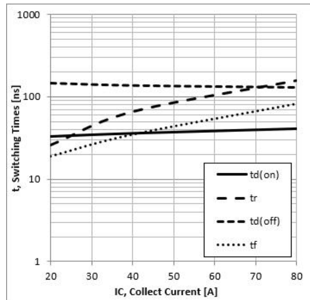
Figure 12: Typical Switching Time VS. IC, TC=25°C, L=100uH, VCE=400V, VGE=15V, RG=15Ω
