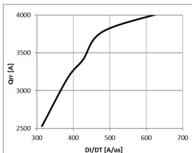
Figure 15: Typical Diode Qrr VS. DI/DT, TC=25°C VCC=600V, VGE=15V, IF=50A
