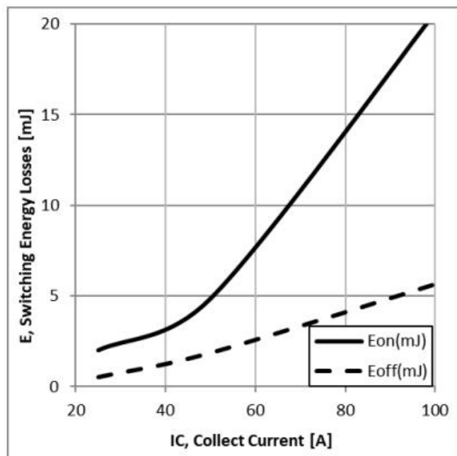
Figure 11: Typical Energy Loss VS. I_C , T_C=25^\circ\text{C} , L=200\mu\text{H} , V_{CE}=600\text{V} , V_{GE}=15\text{V} , R_G=15\Omega
