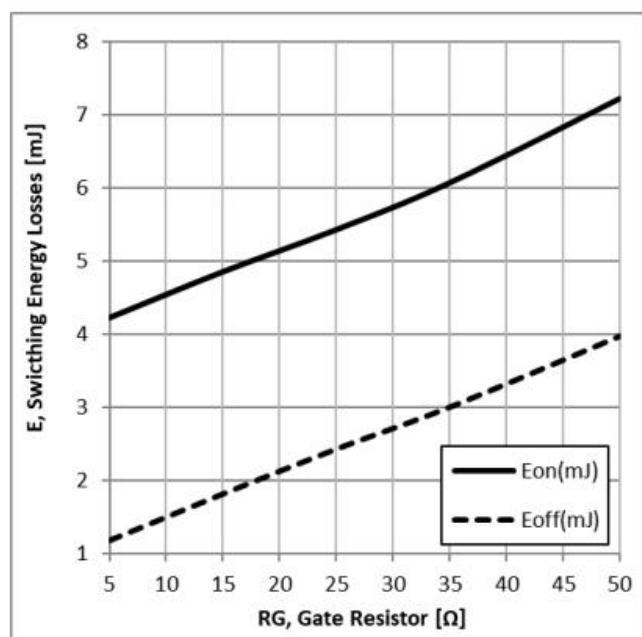
Figure 9: Typical Energy Loss VS. R_G , T_C=25^\circ\text{C} , L=200\mu\text{H} , V_{CE}=600\text{V} , V_{GE}=15\text{V} , I_C=50\text{A}
