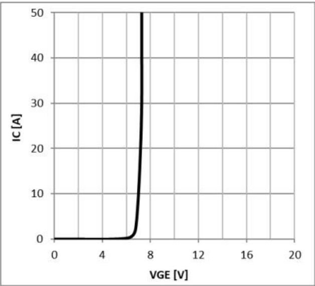
Figure 7: Typical Gate Threshold Voltage
