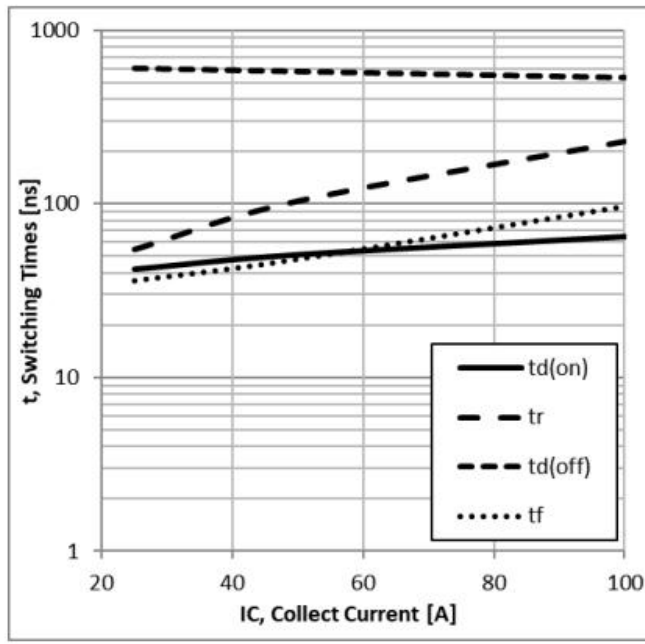
Figure 12: Typical Switching Time VS. I_C , T_C=25^\circ\text{C} , L=200\mu\text{H} , V_{CE}=600\text{V} , V_{GE}=15\text{V} , R_G=15\Omega
