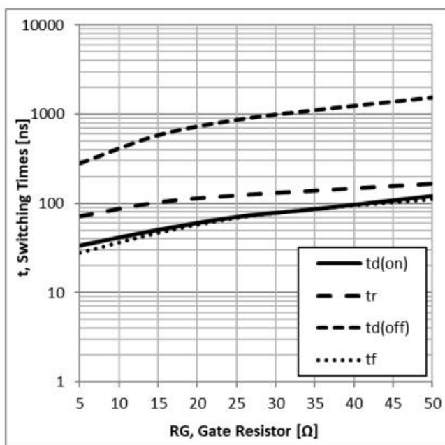
Figure 10: Typical Switching Time VS. R_G , T_C=25^\circ\text{C} , L=200\mu\text{H} , V_{CE}=600\text{V} , V_{GE}=15\text{V} , I_C=50\text{A}
