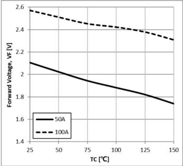
Figure 8: Typical Forward Voltage vs I_F
