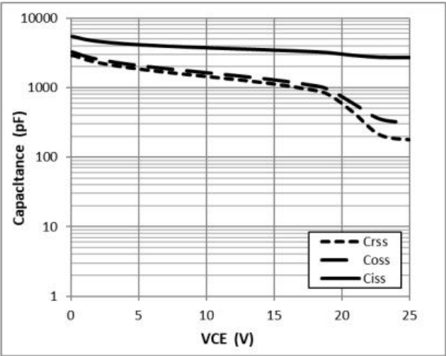
Figure 17: Typical Capacitance VS. VCE, VGE=0V,f=1MHz
