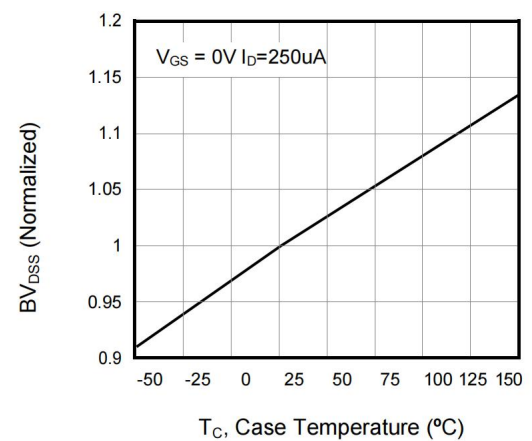
Figure 4. BVDSS Variation vs. Temperature
