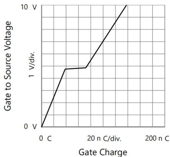
Figure 8. Gate Charge
