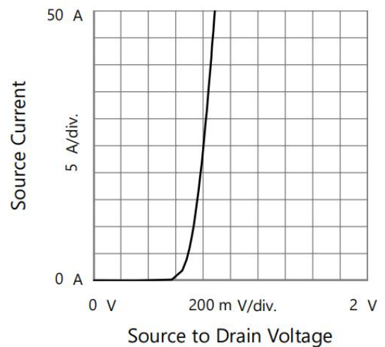
Figure 6. Body Diode Forward Characteristics
