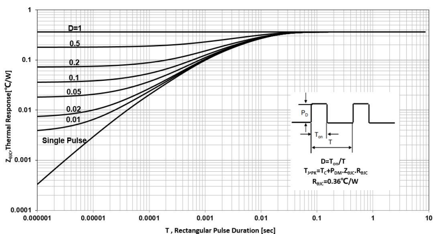
Figure 9. Transient Thermal Impedance
