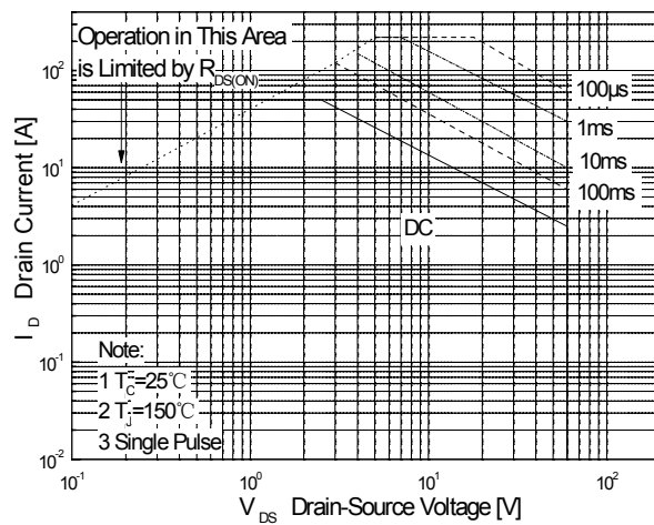
Maximum Safe Operating Area 55N06C/D
