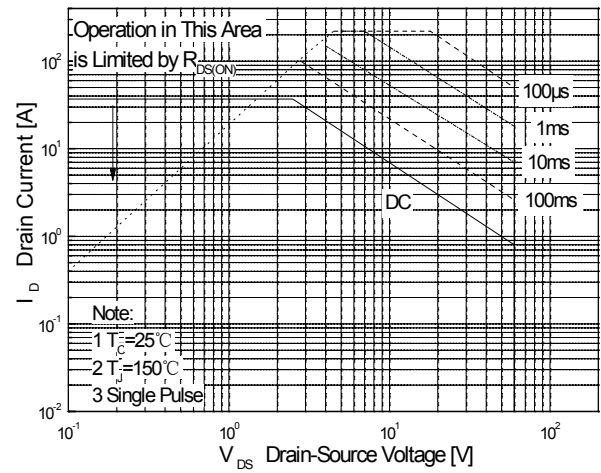
Maximum Safe Operating Area 55N06F
