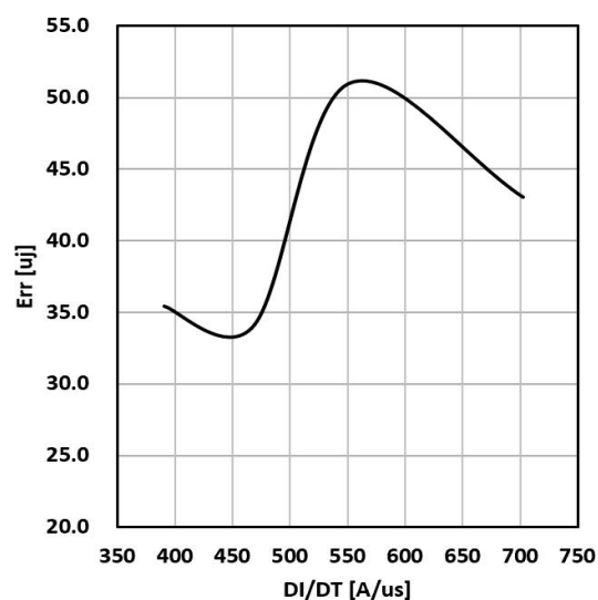
Figure 16. Typical diode Err vs di/dt Tc=25°C VCE=400V VGE=15V IF=5A
