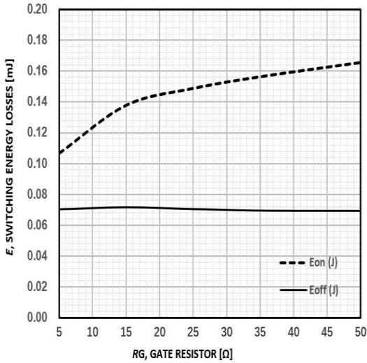
Figure9: Typical energy loss VS. R_g , T_C=25^{\circ}\text{C} , V_{CE}=400\text{V} , V_{GE}=15\text{V} , I_C=5\text{A}
