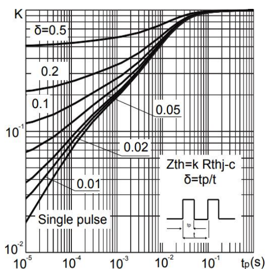
Figure 8. Normalized Maximum Transient Thermal Impedance for IGBT
