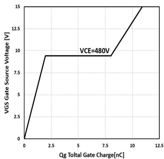
Figure 4: Typical gate charge VS. V_{GS} , I_C=5\text{A}
