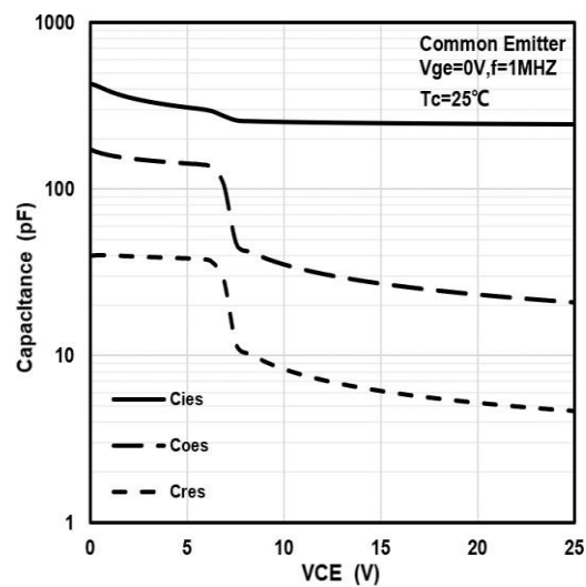
Figure 6. Typical capacitance VS. VCE, V_{GE}=0V, f=1MHz
