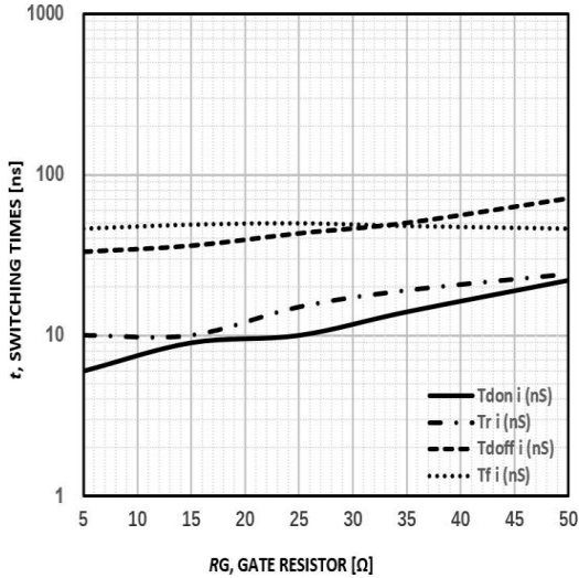
Figure10: Typical switching time VS. R_g , T_C=25^{\circ}\text{C} , V_{CE}=400\text{V} , V_{GE}=15\text{V} , I_C=5\text{A}
