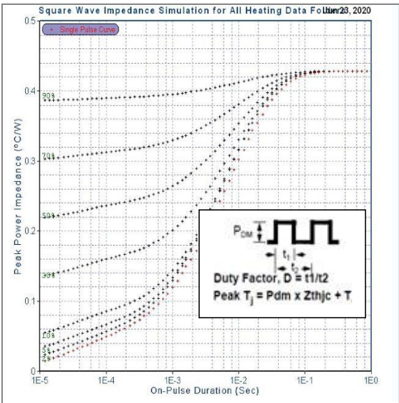
Figure 20. Transient Thermal Impedance of FRD
