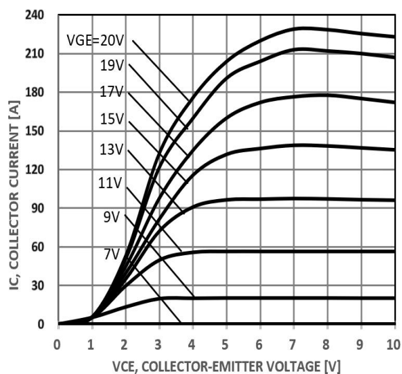
Figure 1. Typical Output Characteristics, T_c = 25^\circ\text{C}
