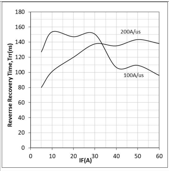
Figure 16. Reverse Recovery Time, Tc=25°C
