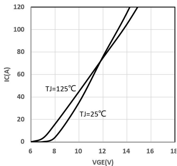
Figure 2. Transfer Characteristics
