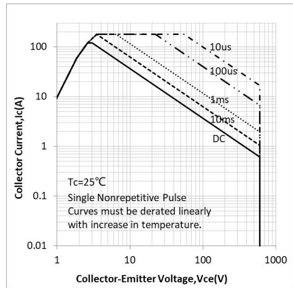
Figure 6. SOA Characteristics
