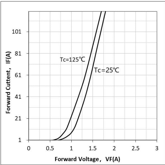
Figure 14. Forward Characteristics
