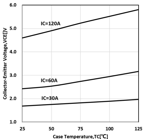
Figure 3. Saturation Voltage vs. Case Temperature, Common Emitter, V_{GE} = 15\text{V}
