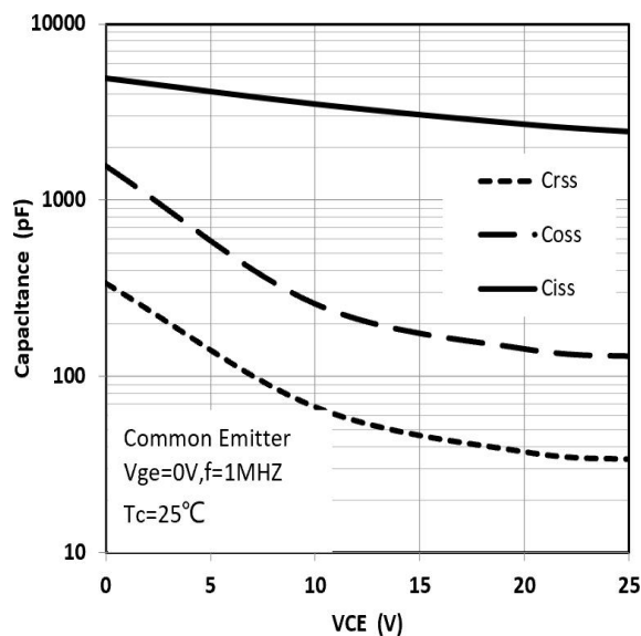
Figure 4. Capacitance Characteristics, Common Emitter, V_{GE} = 0\text{V} , f = 1\text{MHz} , T_c = 25^\circ\text{C}
