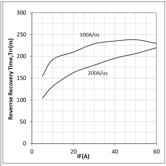
Figure 18. Reverse Recovery Time, T_c=125^{\circ}C
