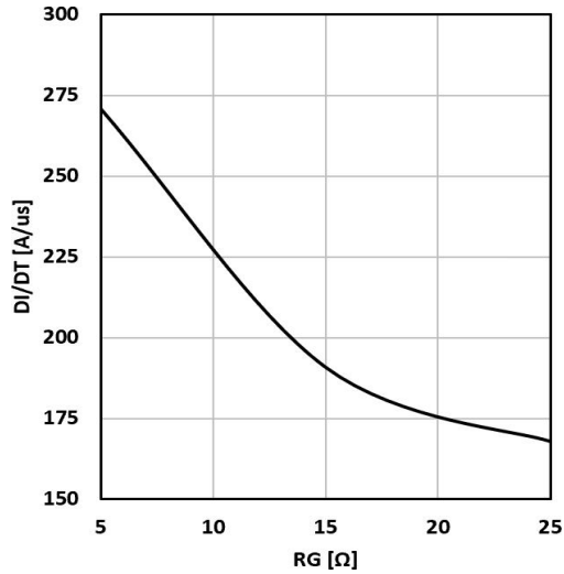
Figure 13. Typical diode di/dt vs rg Tc=25°C VCE=600V VGE=15V IF=75A
