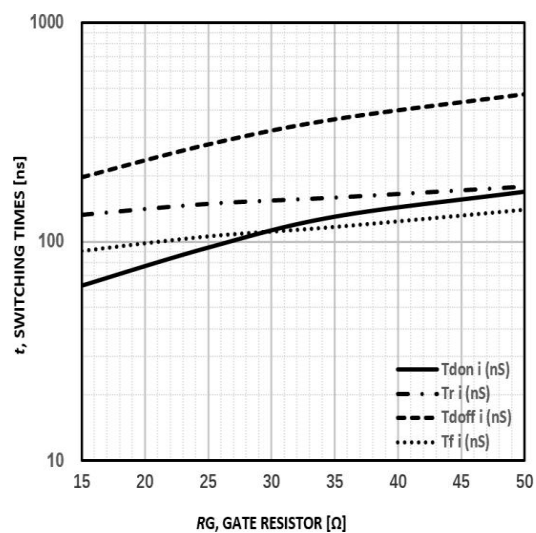
Figure10: Typical switching time VS. Rg, TC=25°C, VCE=400V, VGE=15V ,IC=75A
