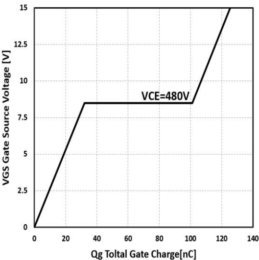
Figure 4: Typical gate charge VS. VGE, IC=75A
