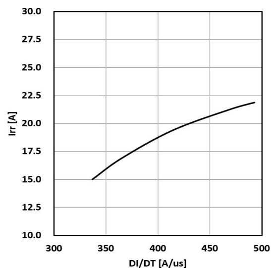
Figure 14. Typical diode irr vs di/dt Tc=25°C VCE=400V VGE=15V IF=75A
