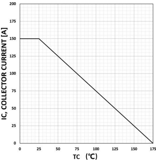
Figure 1. Maximum DC collector current VS. case temperature
