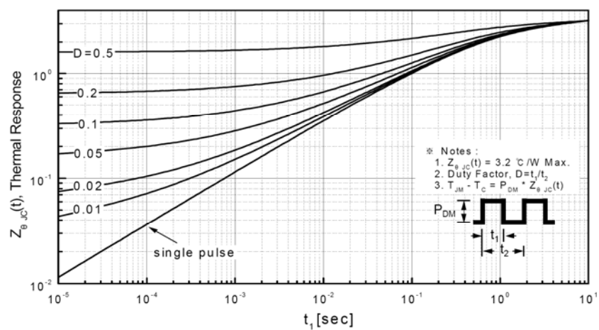
Transient Thermal Response Curve For 8N65F
