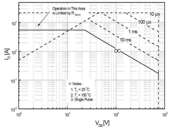
Maximum Safe Operating Area For 8N65F
