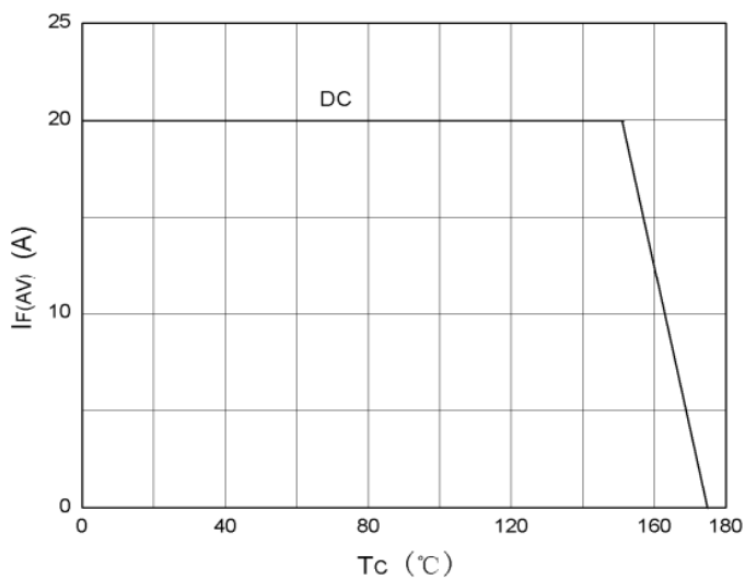
I_F(\text{AV}) vs T_C
