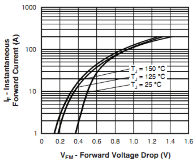
Fig. 1 - Maximum Forward Voltage Drop Characteristics (Per Leg)
