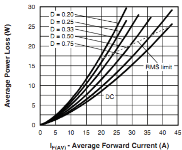
Fig. 4 - Forward Power Loss Characteristics (Per Leg)
