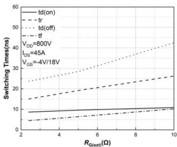
Figure 26. Switching Times vs. R_{G(ext)} T_J = 175^\circ\text{C}
