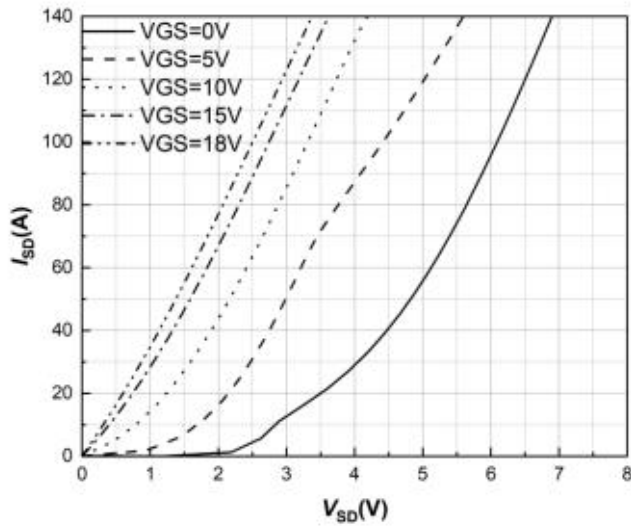
Figure 13. 3rd Quadrant Characteristic T_j = -55^\circ\text{C}
