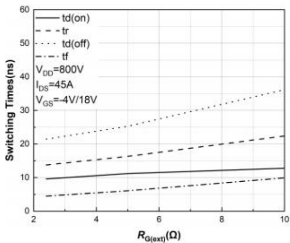
Figure 25. Switching Times vs. R_{G(ext)} T_J = 25^\circ\text{C}
