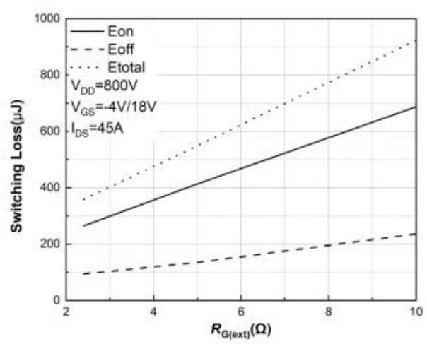
Figure 24. Clamped Inductive Switching Energy vs. R_{G(\text{ext})} T_j=175^{\circ}\text{C}
