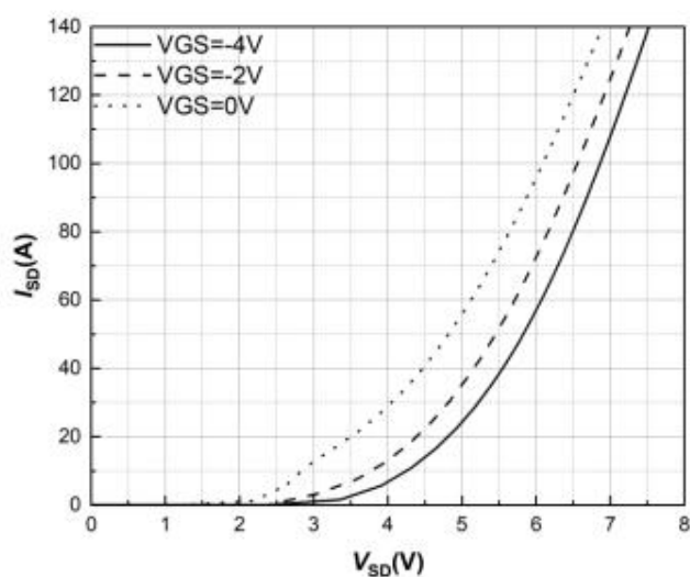
Figure 8. Body Diode Characteristic T_J = -55^\circ\text{C}
