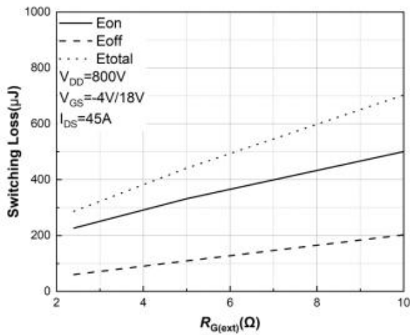
Figure 23. Clamped Inductive Switching Energy vs. R_{G(\text{ext})} T_j=25^{\circ}\text{C}
