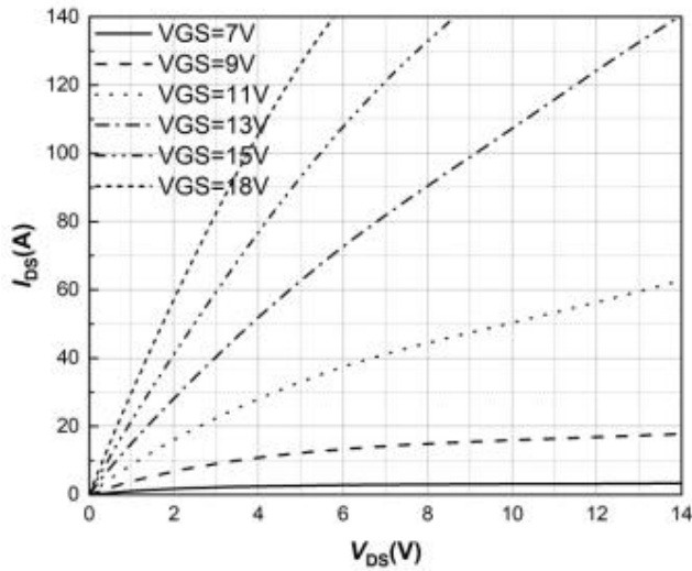
Figure 1. Output Characteristics T_j = -55^{\circ}\text{C}
