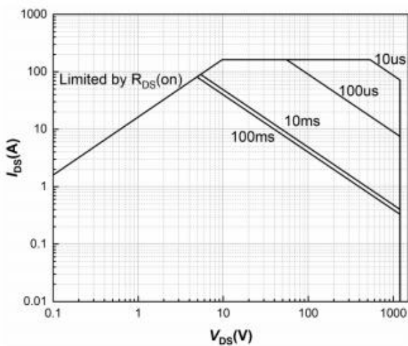
Figure 27. Safe Operating Area
