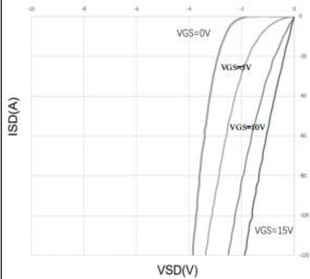
Diagram 10: 3rd Quadrant Characteristic at 25 °C
