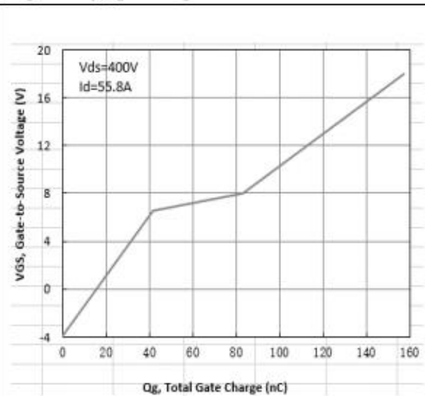
Diagram 4: Typ. gate charge
