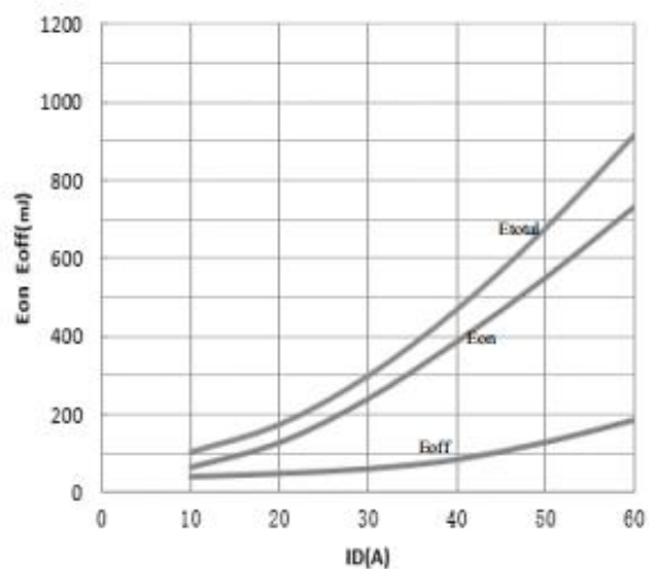
Diagram 13: Clamped Inductive Switching Energy vs. Drain Current (VDD = 400V)
