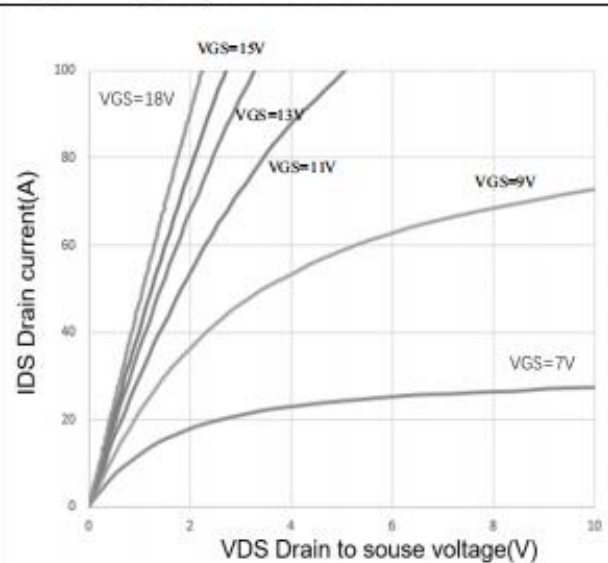
Diagram 2: Typ. output characteristics
