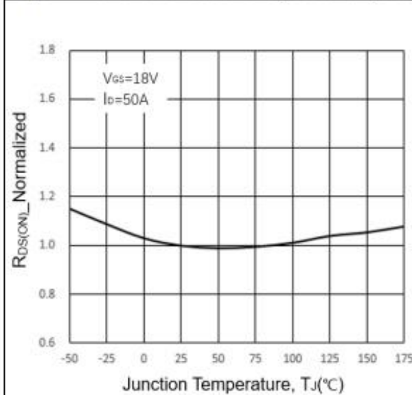
Diagram 7: Normalized on-resistance vs. junction temperature
