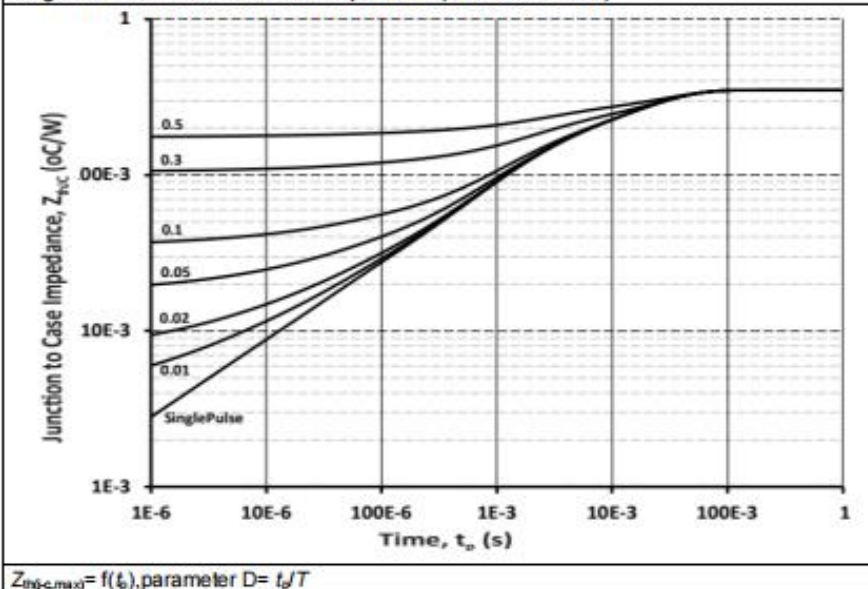
Diagram 19: Transient Thermal Impedance (Junction - Case)
