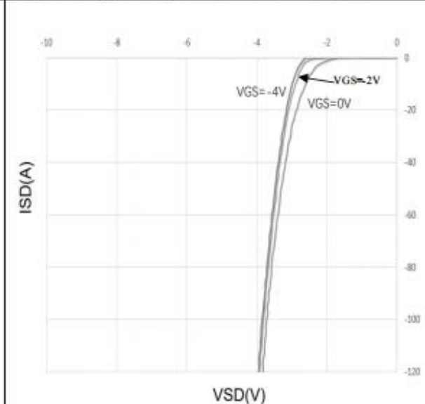
Diagram 8: Typical body diodes Characteristics at 25°C
