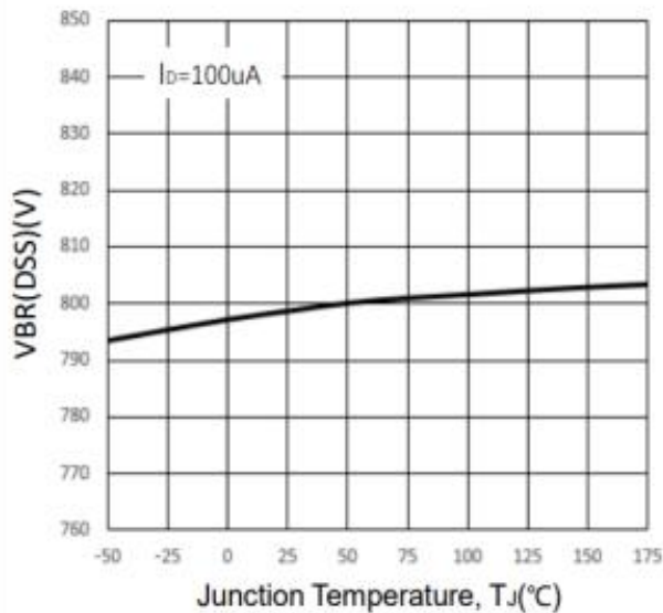
Diagram 9: BVDSS VS junction temperature
