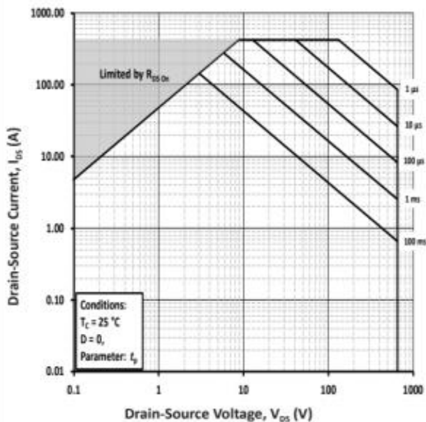
Diagram 11: Safe operating area(SOA)
